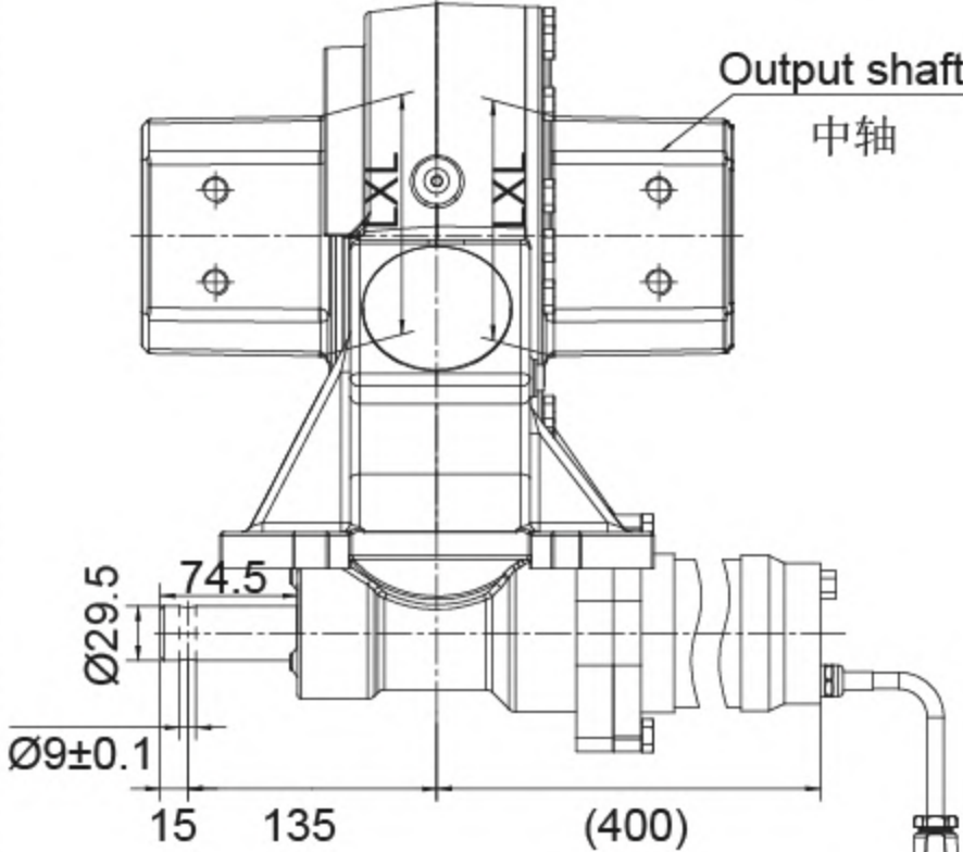
SIDE VIEW 侧视图
