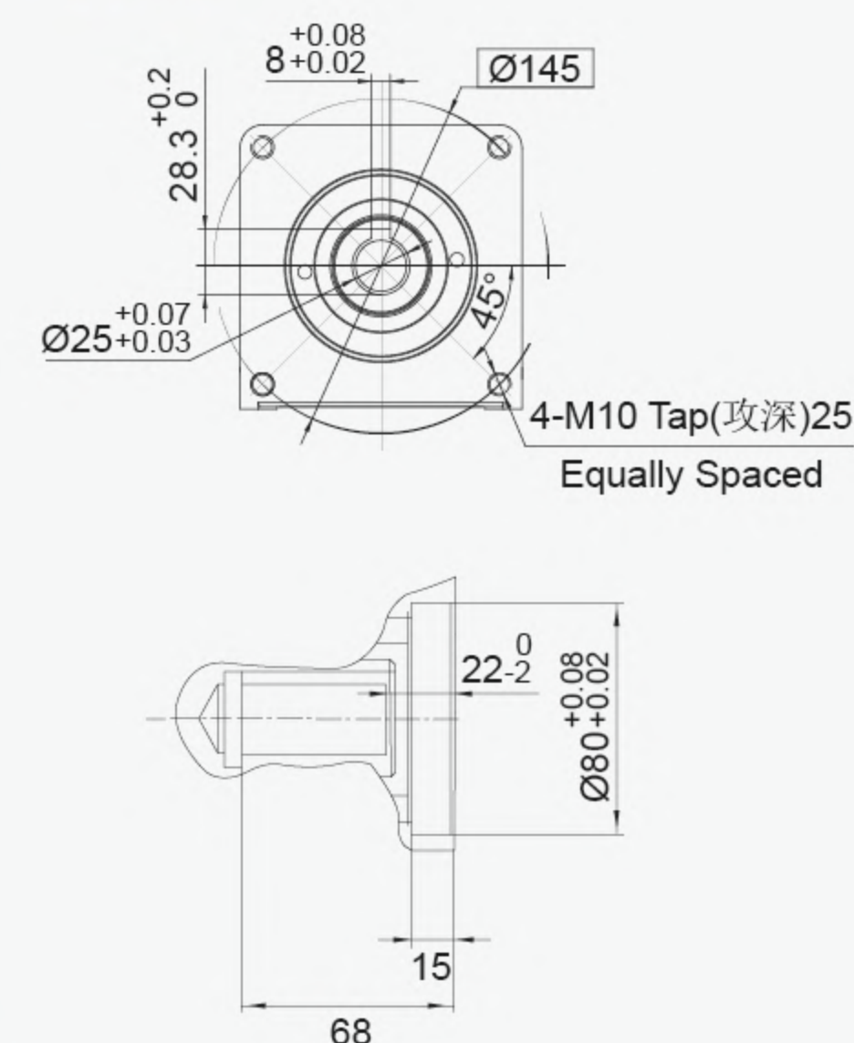
VIEW A A向视图
