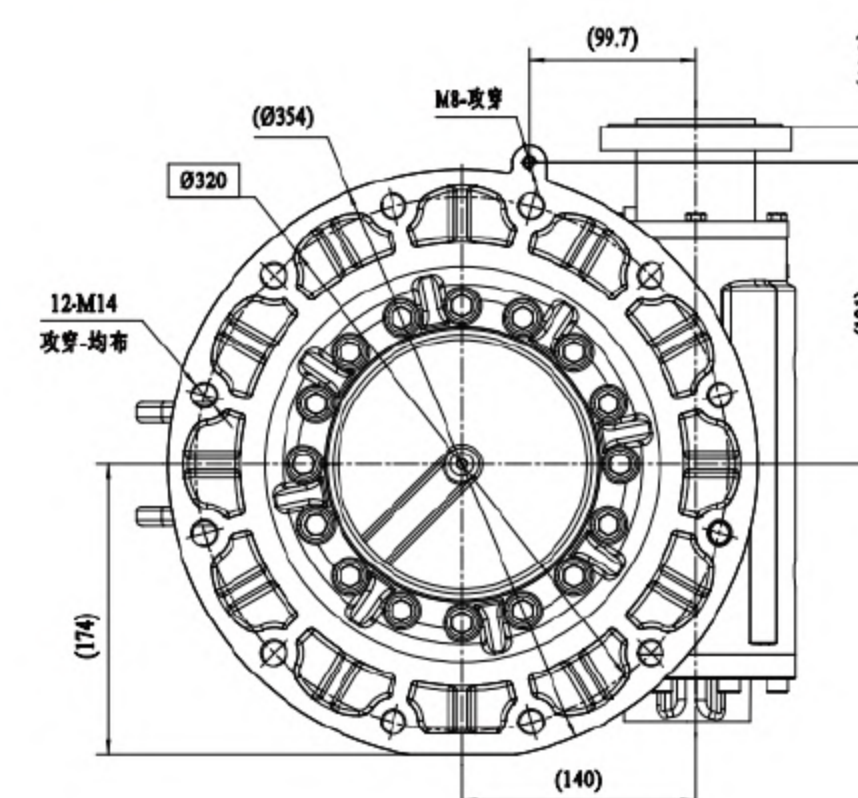
VIEW C OPTION C向选项
