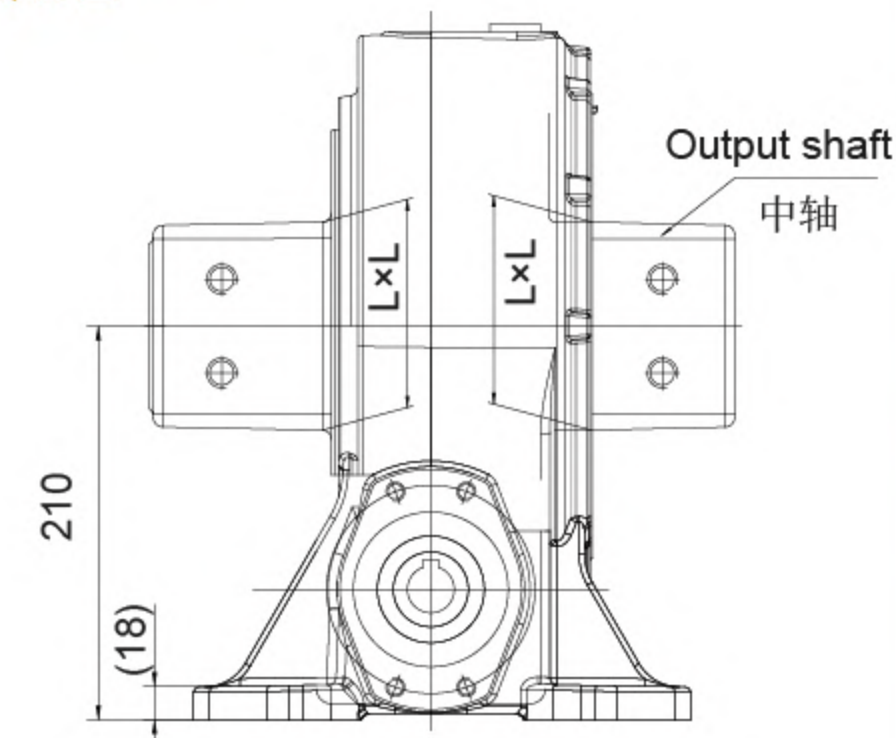
SIDE VIEW 侧视图
