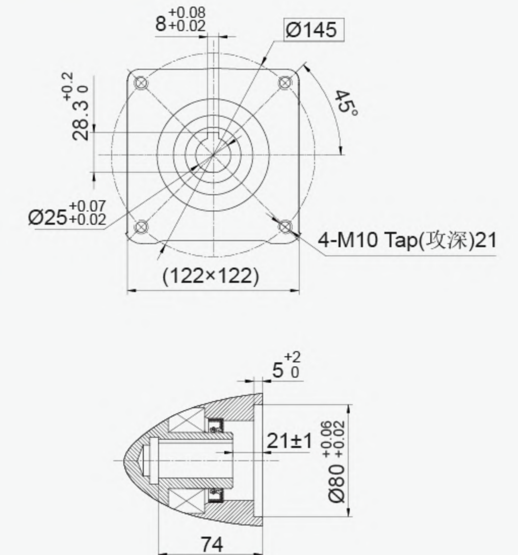
VIEW A A向视图
