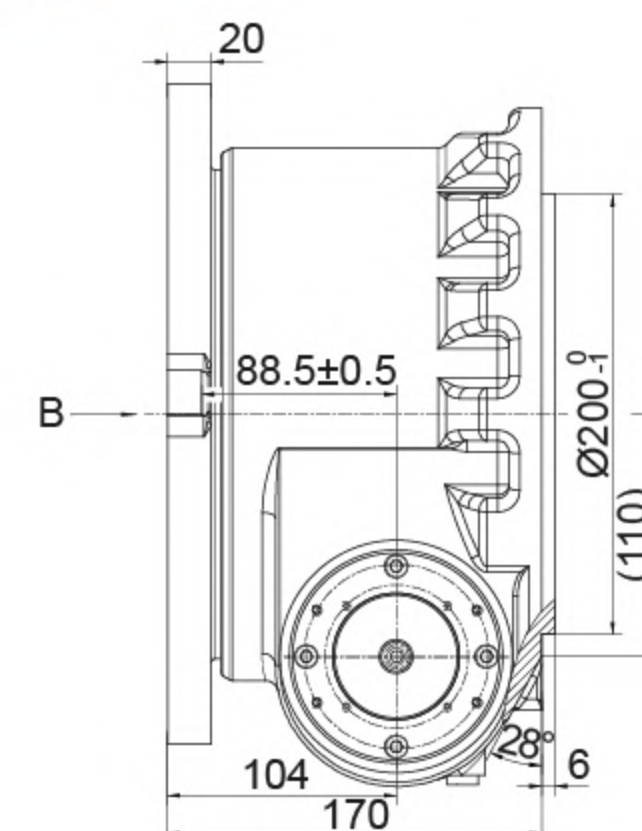
SIDE VIEW 侧视图
