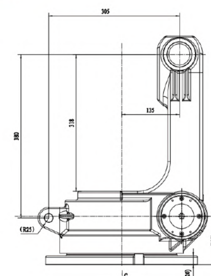
SIDE VIEW 侧视图
