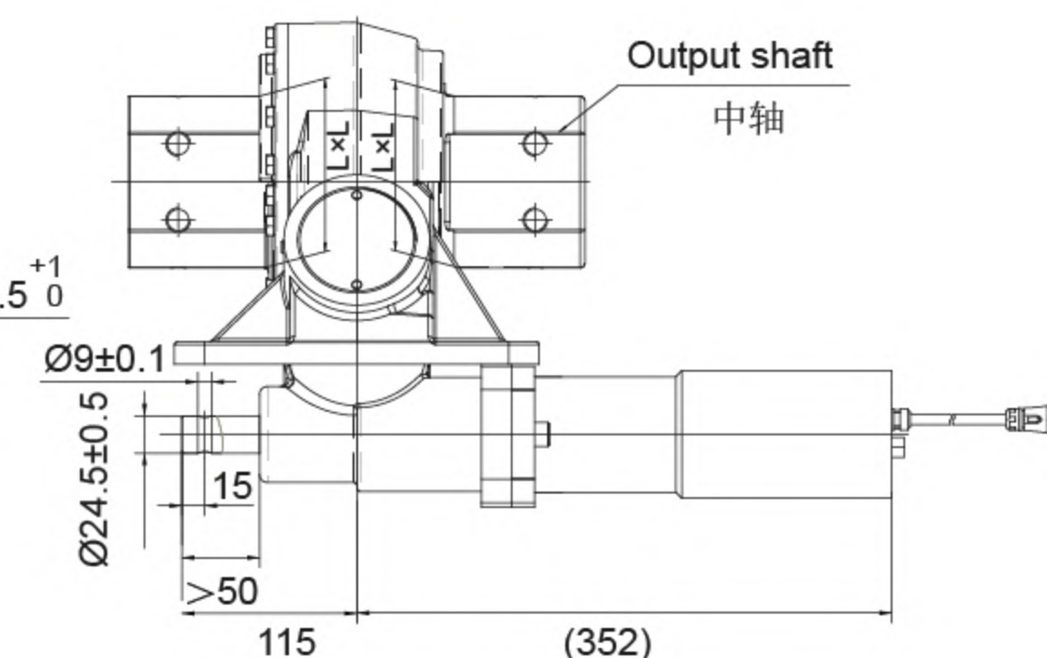
VIEW A A向视图
