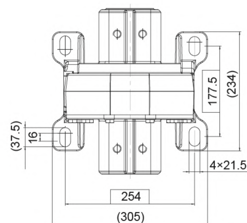
SIDE VIEW 侧视图
