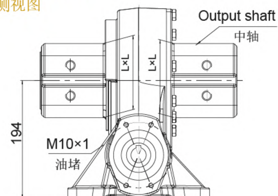
SIDE VIEW 侧视图
