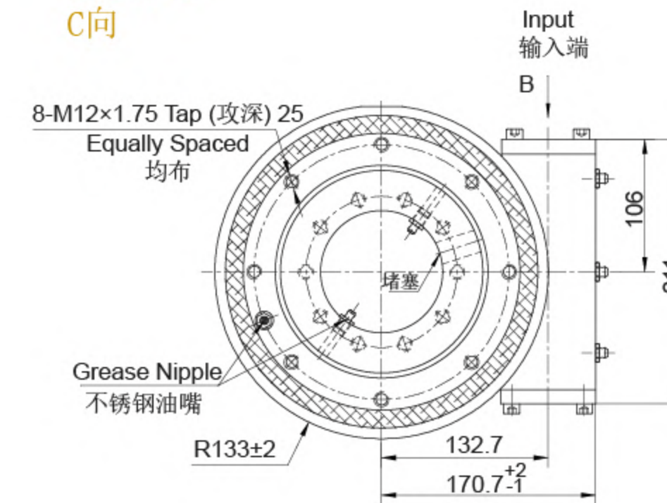
VIEW A A向视图
