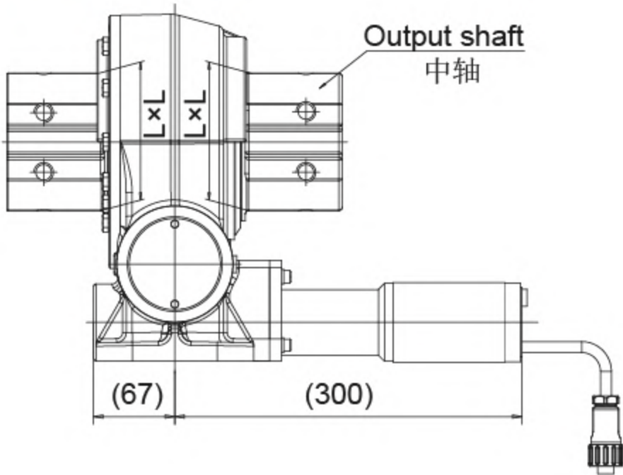
SIDE VIEW 侧视图
