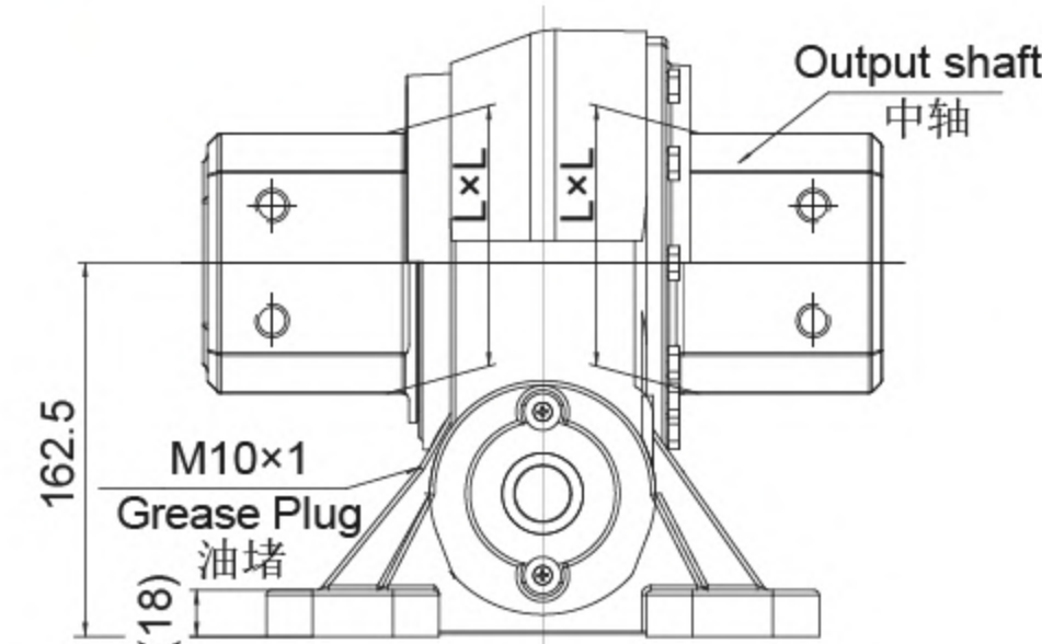
SIDE VIEW 侧视图
