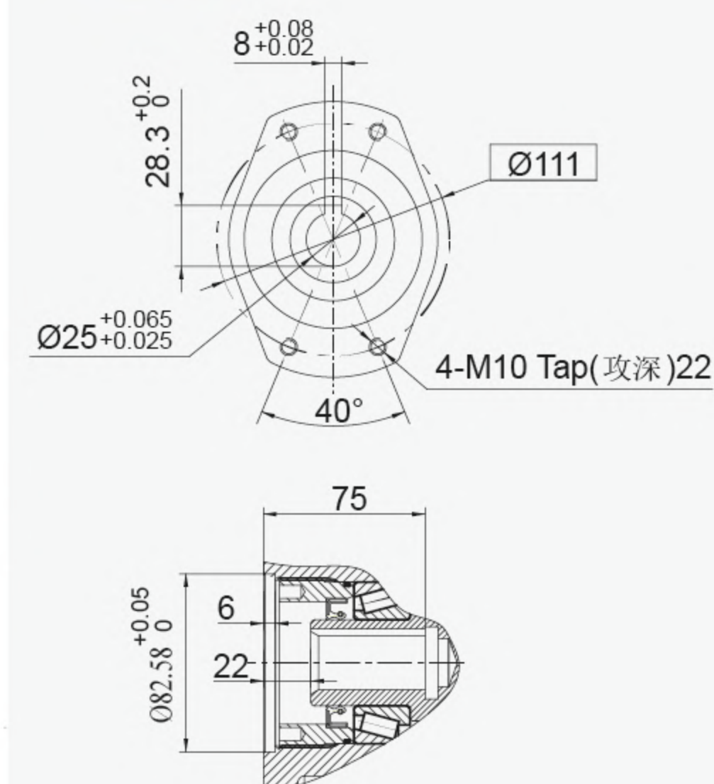
VIEW A A向视图
