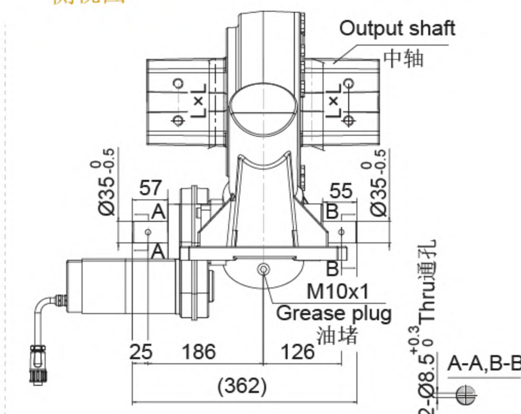
SIDE VIEW 侧视图
