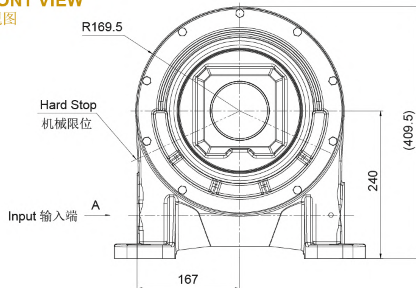
FRONT VIEW
