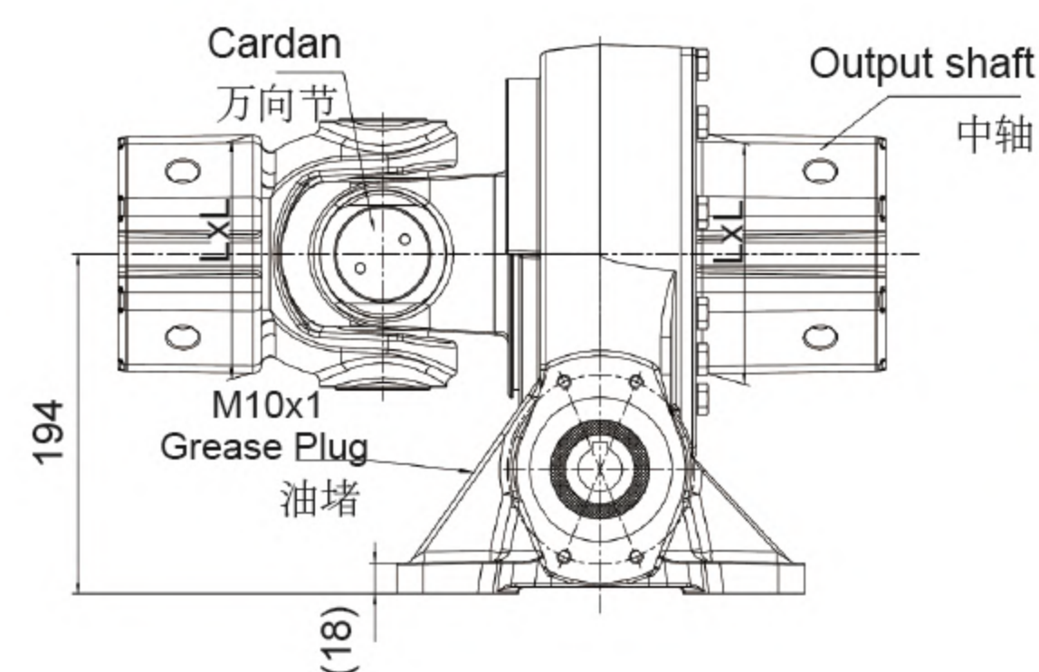
SIDE VIEW 侧视图
