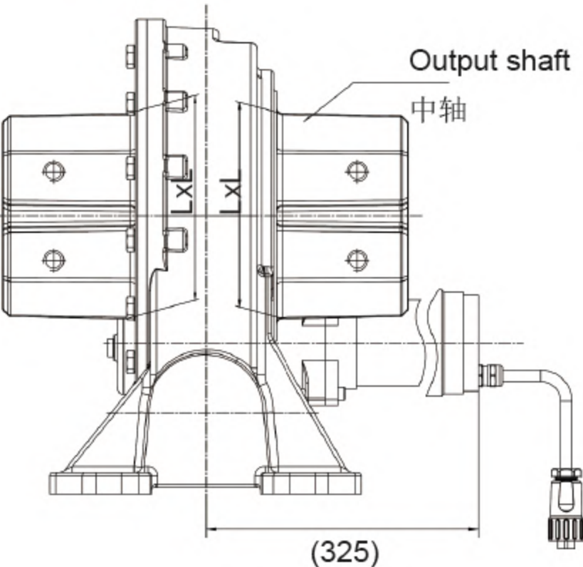
SIDE VIEW 侧视图
