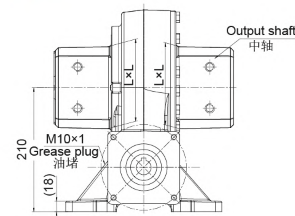
SIDE VIEW 侧视图
