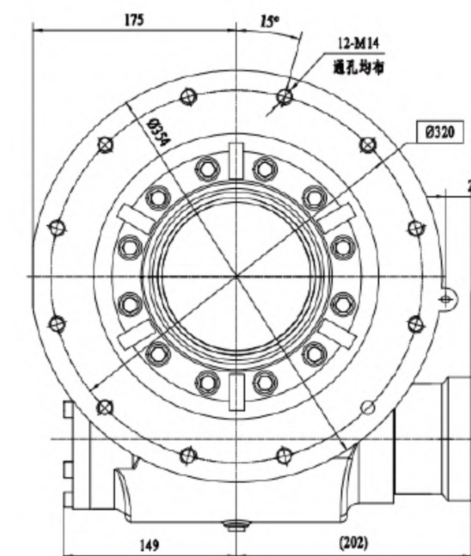
VIEW B OPTION B向选项
