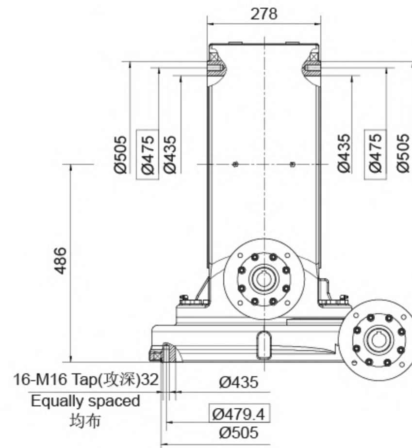
SIDE VIEW 侧视图
