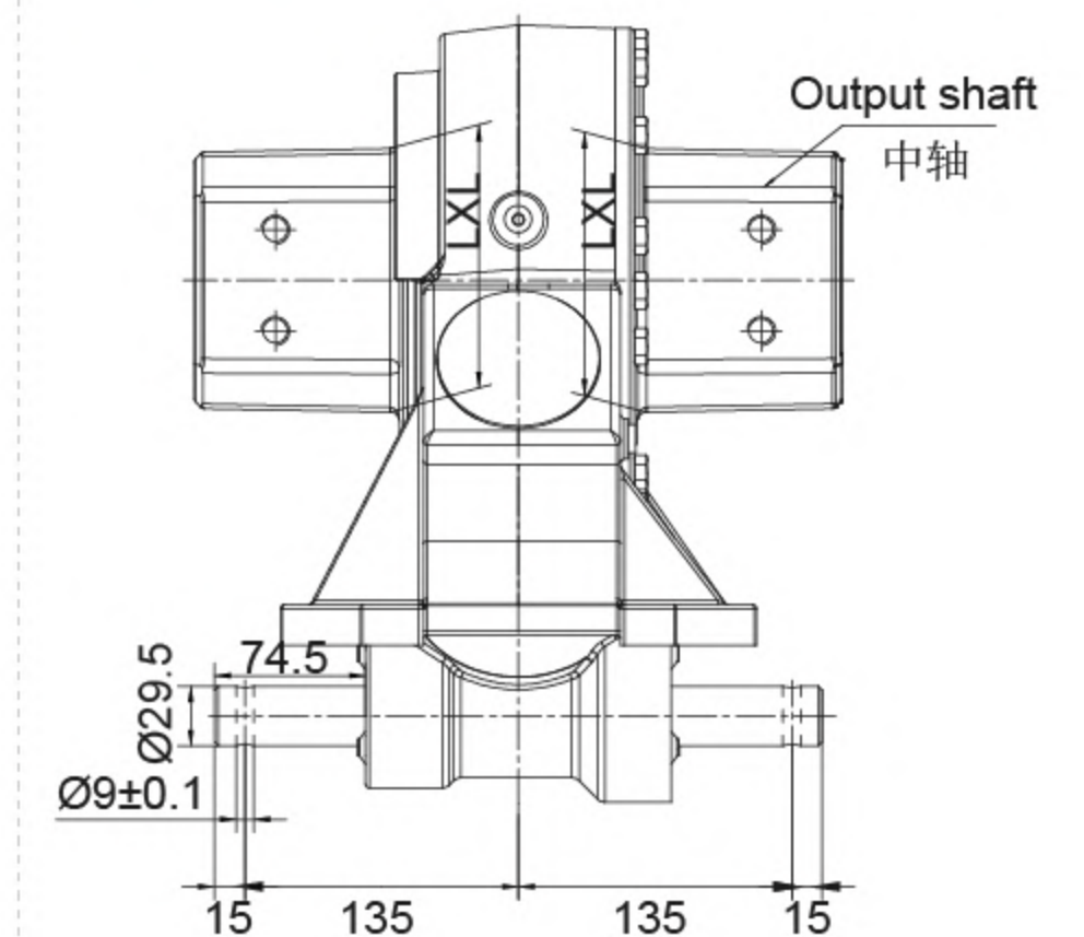
SIDE VIEW 侧视图
