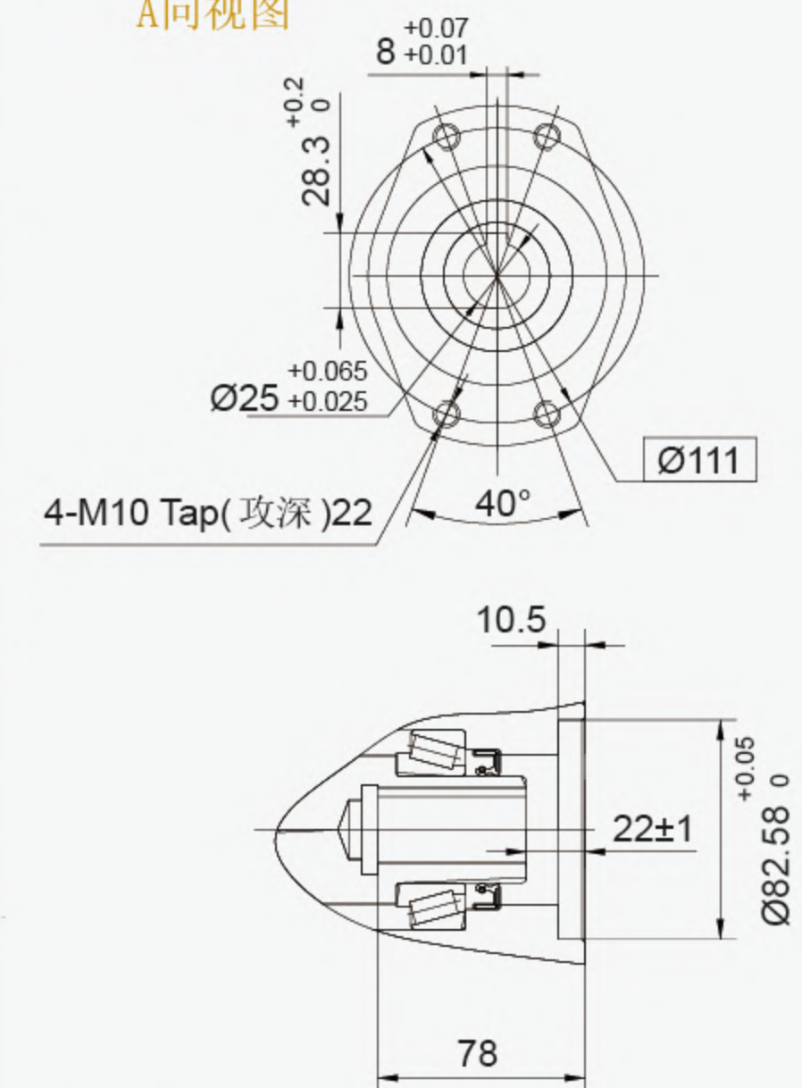
VIEW A A向视图
