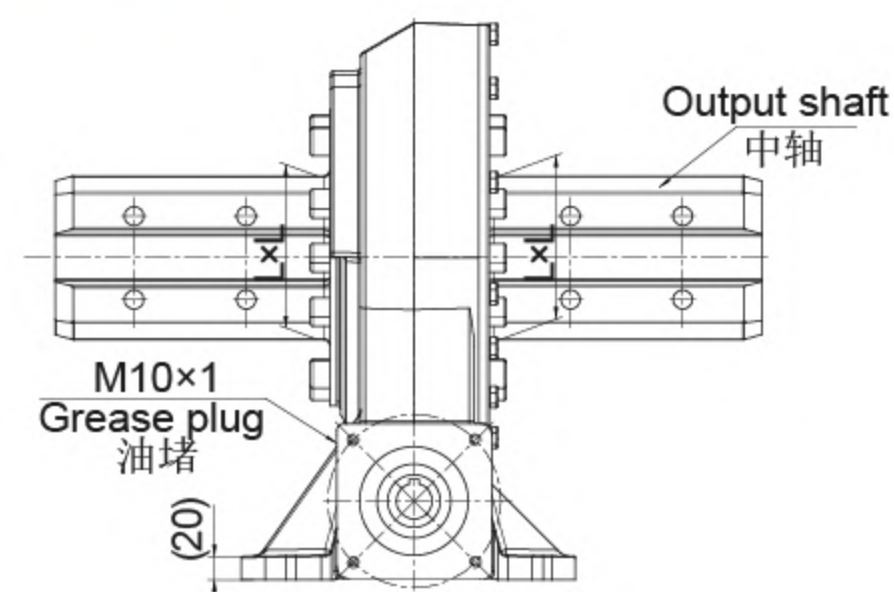
SIDE VIEW 侧视图
