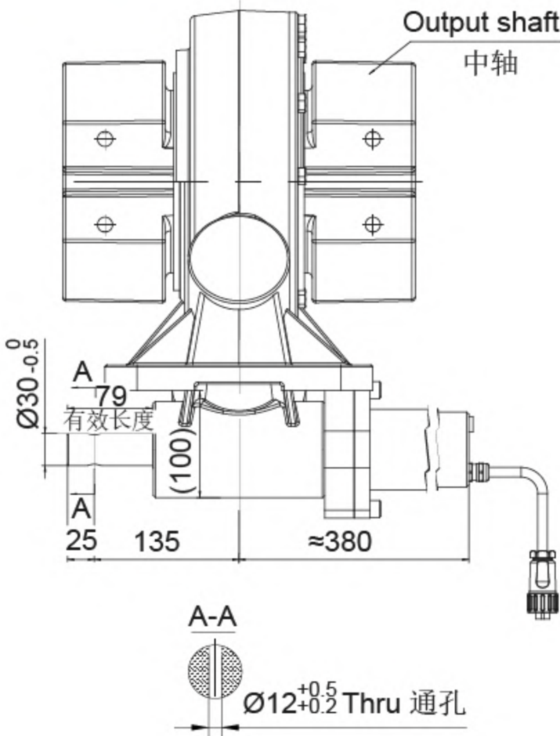
SIDE VIEW 侧视图
