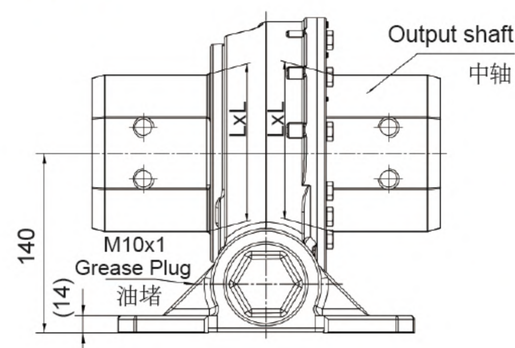
SIDE VIEW 侧视图
