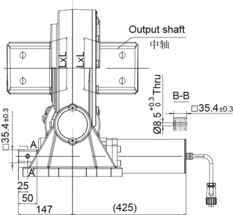
SIDE VIEW 侧视图
