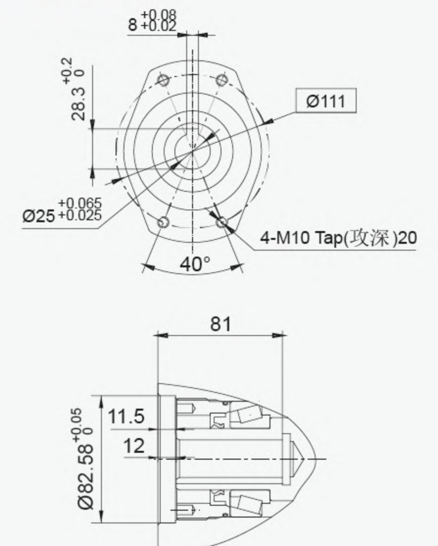
VIEW A A向视图
